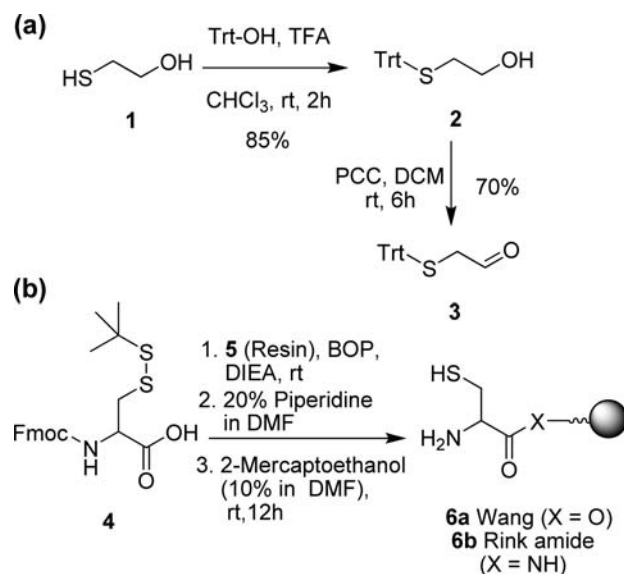
Scheme 1. Preparation of starting Materials for Synthesis of Peptide Thioesters
